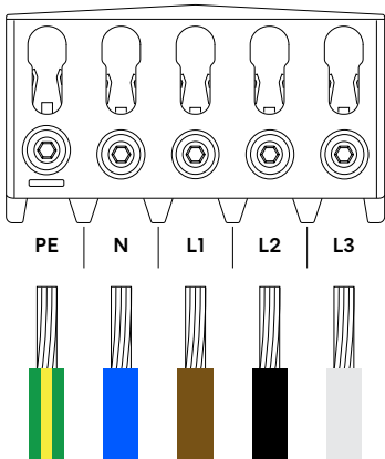
TN/TT 3-fas (230/400 V)
